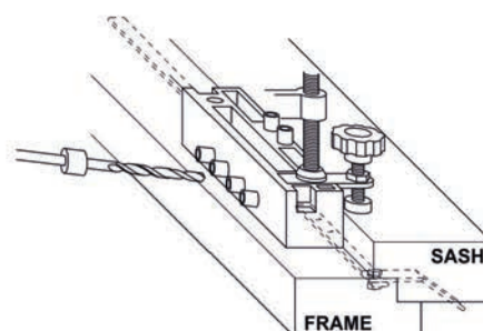
Drilling diagram
